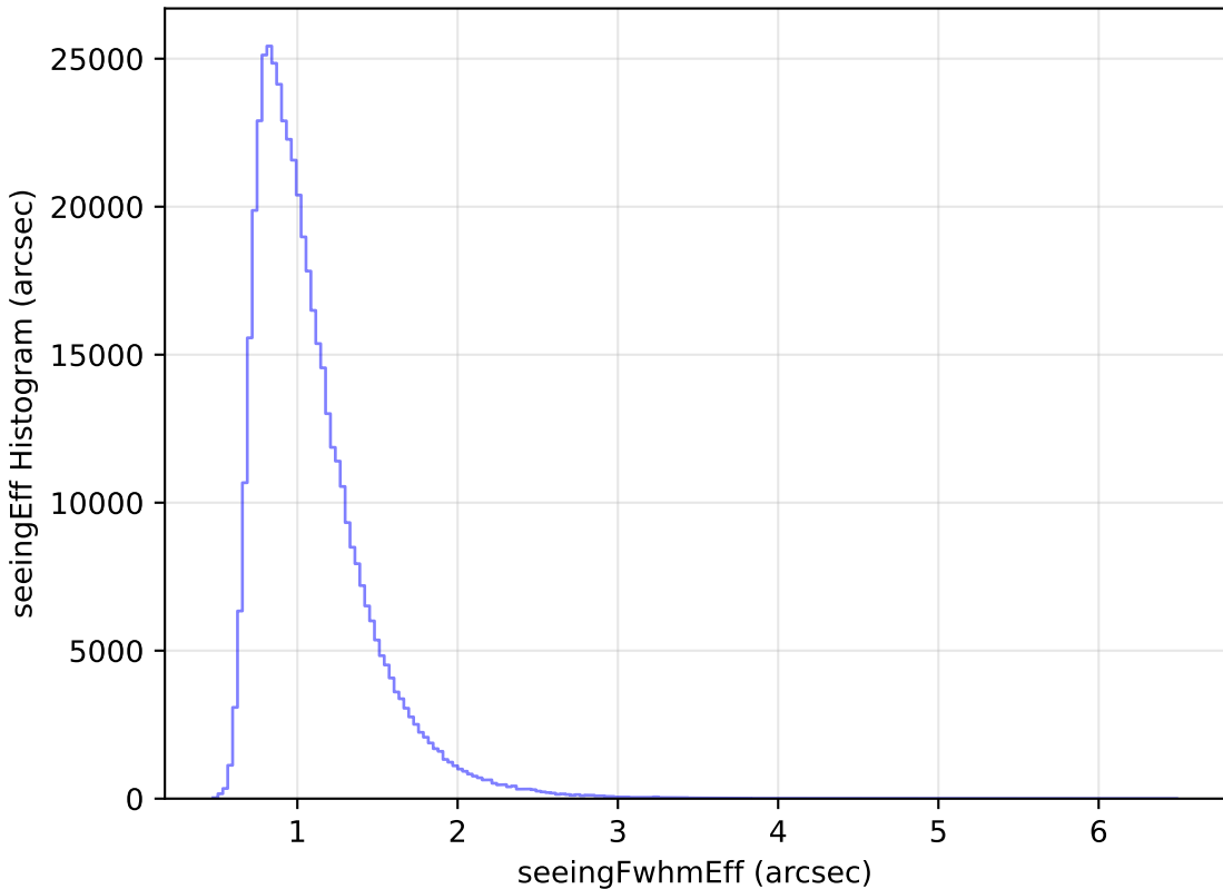
ddf_loaded_half_fl1_v3.4_10yrs WFD i band: seeingEff Histogram
