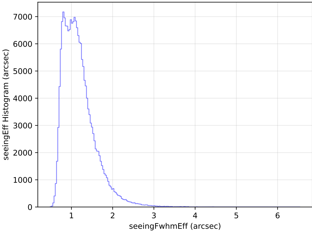
ddf_loaded_half_fl1_v3.4_10yrs WFD g band: seeingEff Histogram
