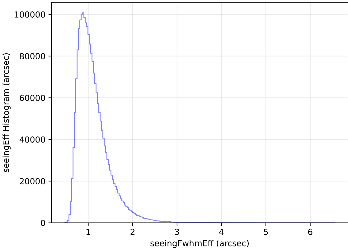
ddf_loaded_half_fl1_v3.4_10yrs WFD all bands: seeingEff Histogram
