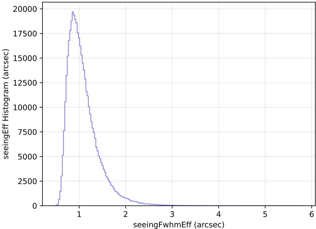
ddf_loaded_half_fl1_v3.4_10yrs All sky z band: seeingEff Histogram
