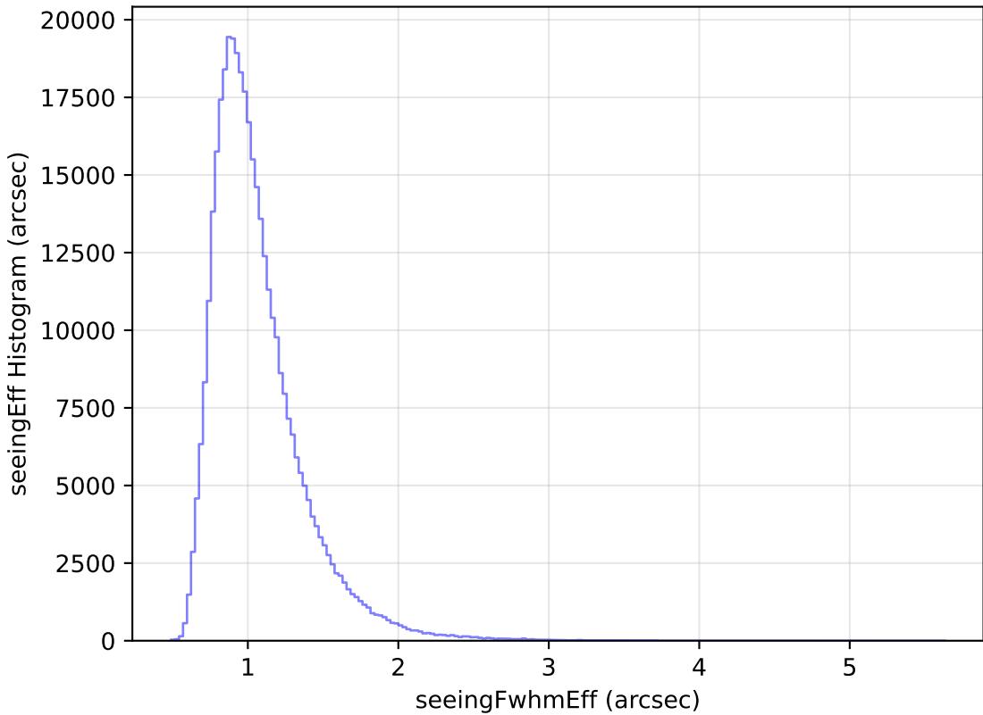
ddf_loaded_half_fl1_v3.4_10yrs All sky y band: seeingEff Histogram
