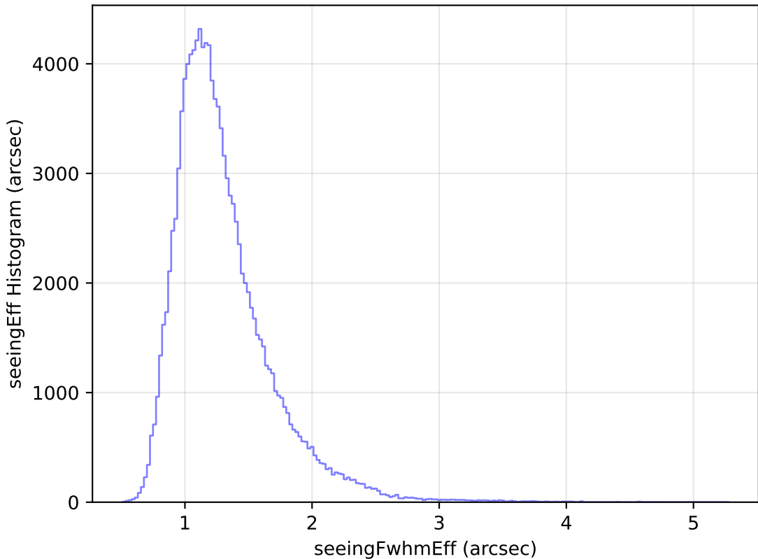
ddf_loaded_half_fl1_v3.4_10yrs All sky u band: seeingEff Histogram
