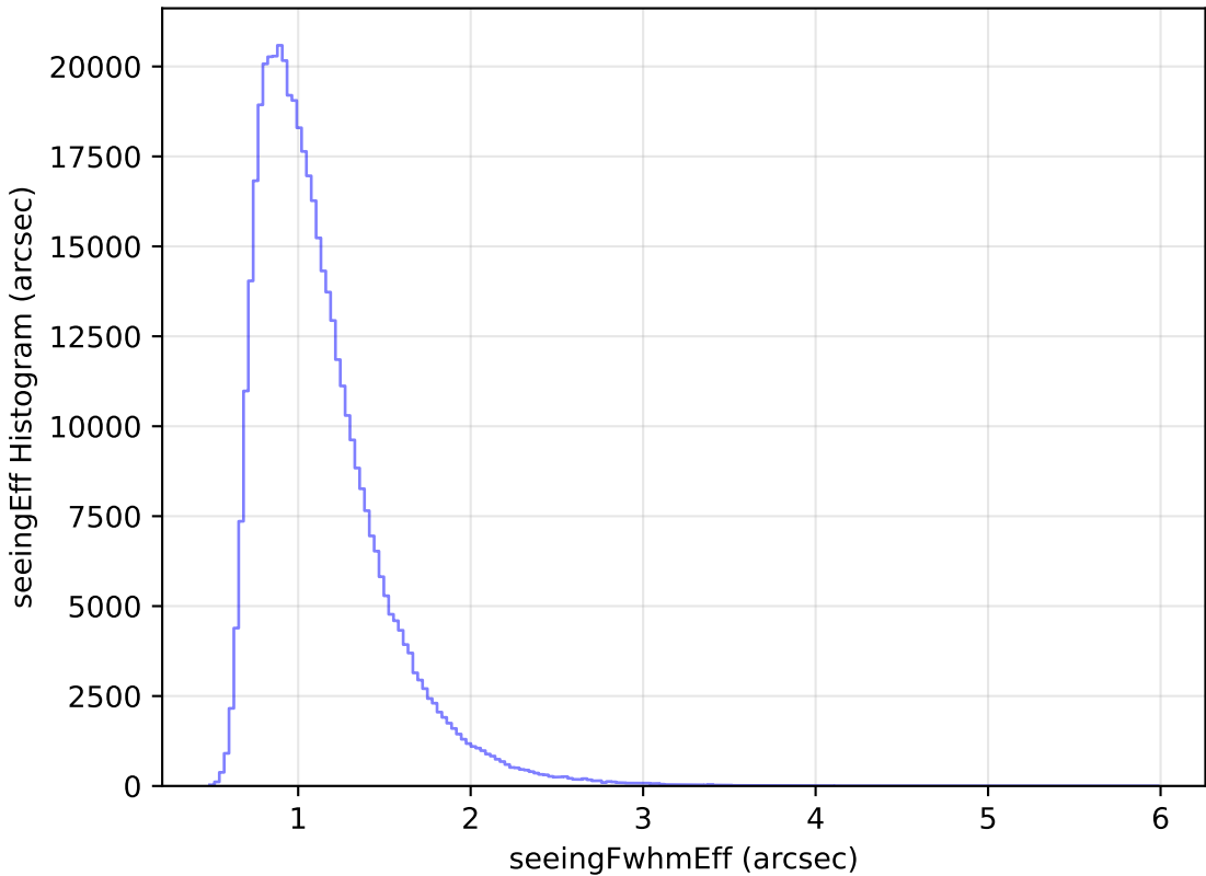
ddf_loaded_half_fl1_v3.4_10yrs All sky r band: seeingEff Histogram
