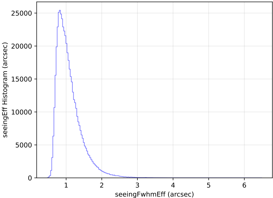
ddf_loaded_half_fl1_v3.4_10yrs All sky i band: seeingEff Histogram
