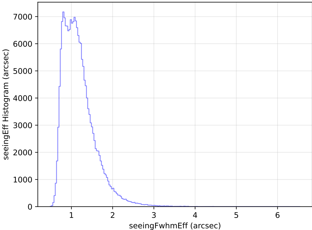
ddf_loaded_half_fl1_v3.4_10yrs All sky g band: seeingEff Histogram
