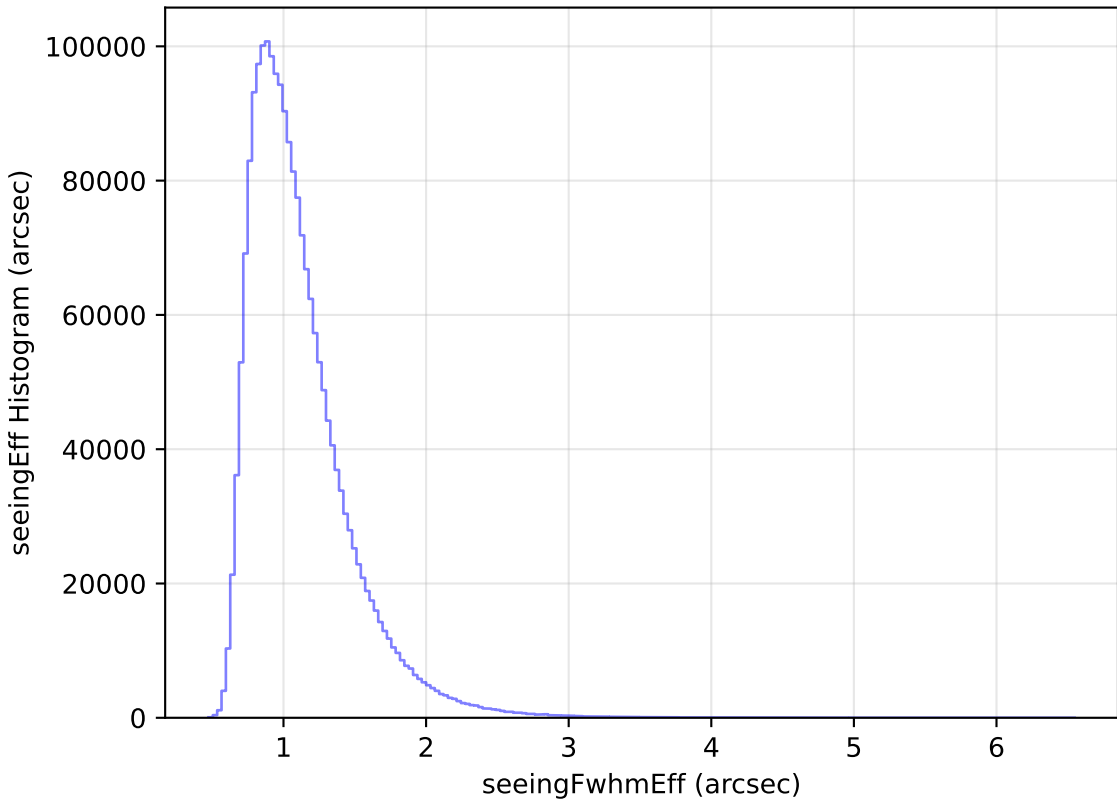
ddf_loaded_half_fl1_v3.4_10yrs All sky all bands: seeingEff Histogram
