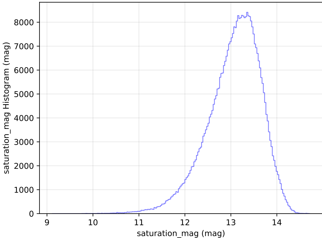
ddf_loaded_half_fl1_v3.4_10yrs WFD y band: saturation_mag Histogram
