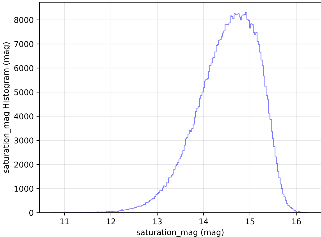
ddf_loaded_half_fl1_v3.4_10yrs WFD r band: saturation_mag Histogram
