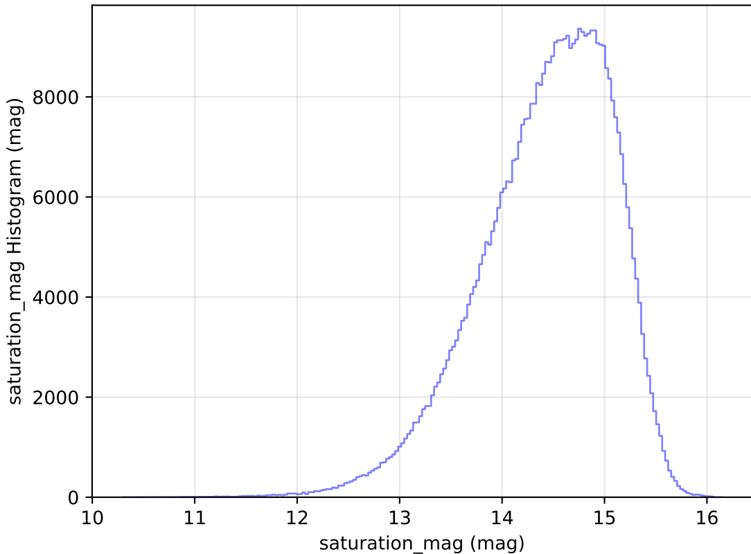
ddf_loaded_half_fl1_v3.4_10yrs WFD i band: saturation_mag Histogram
