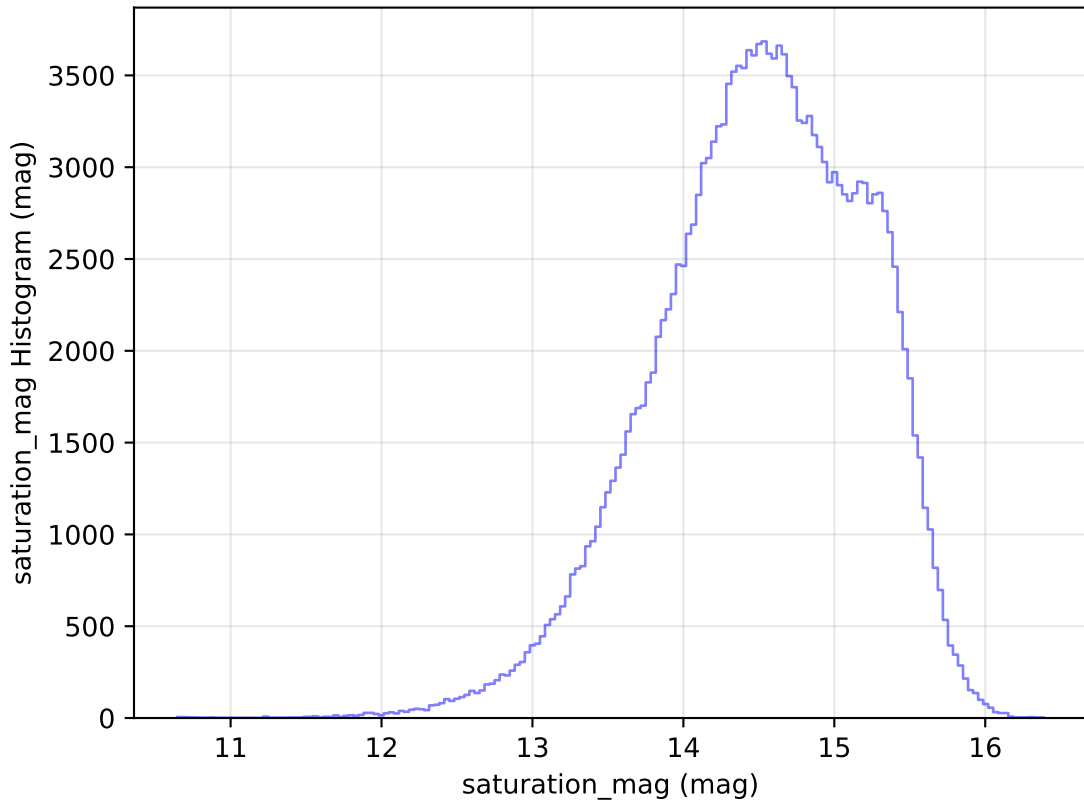
ddf_loaded_half_fl1_v3.4_10yrs WFD g band: saturation_mag Histogram
