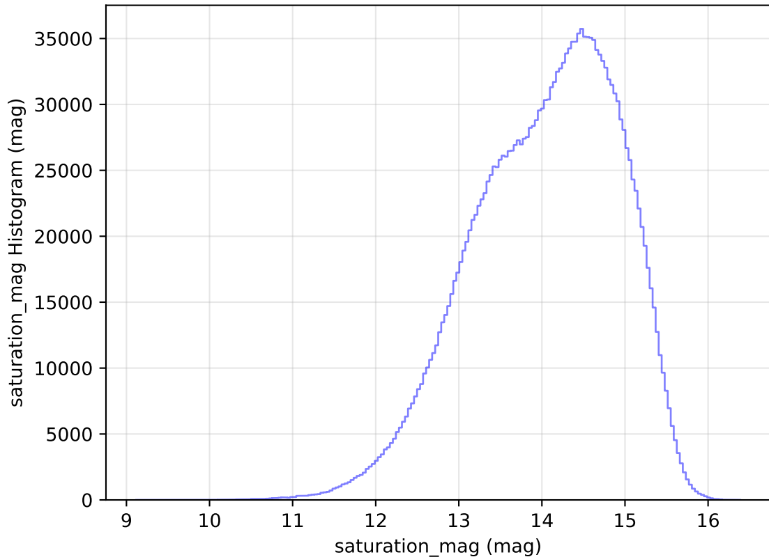
ddf_loaded_half_fl1_v3.4_10yrs WFD all bands: saturation_mag Histogram
