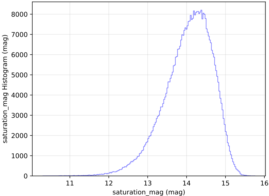
ddf_loaded_half_fl1_v3.4_10yrs All sky z band: saturation_mag Histogram
