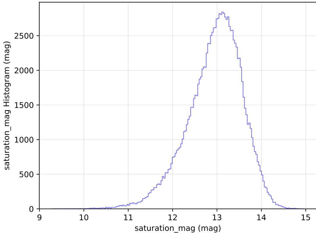
ddf_loaded_half_fl1_v3.4_10yrs All sky u band: saturation_mag Histogram
