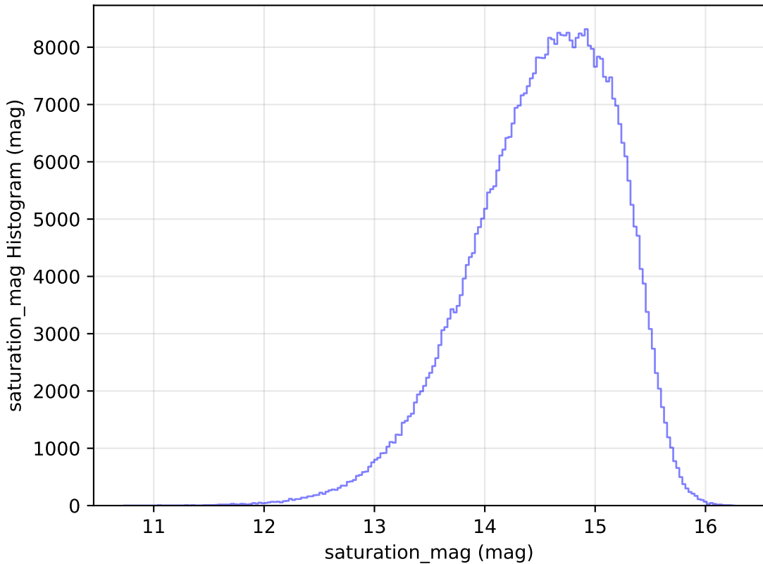
ddf_loaded_half_fl1_v3.4_10yrs All sky r band: saturation_mag Histogram
