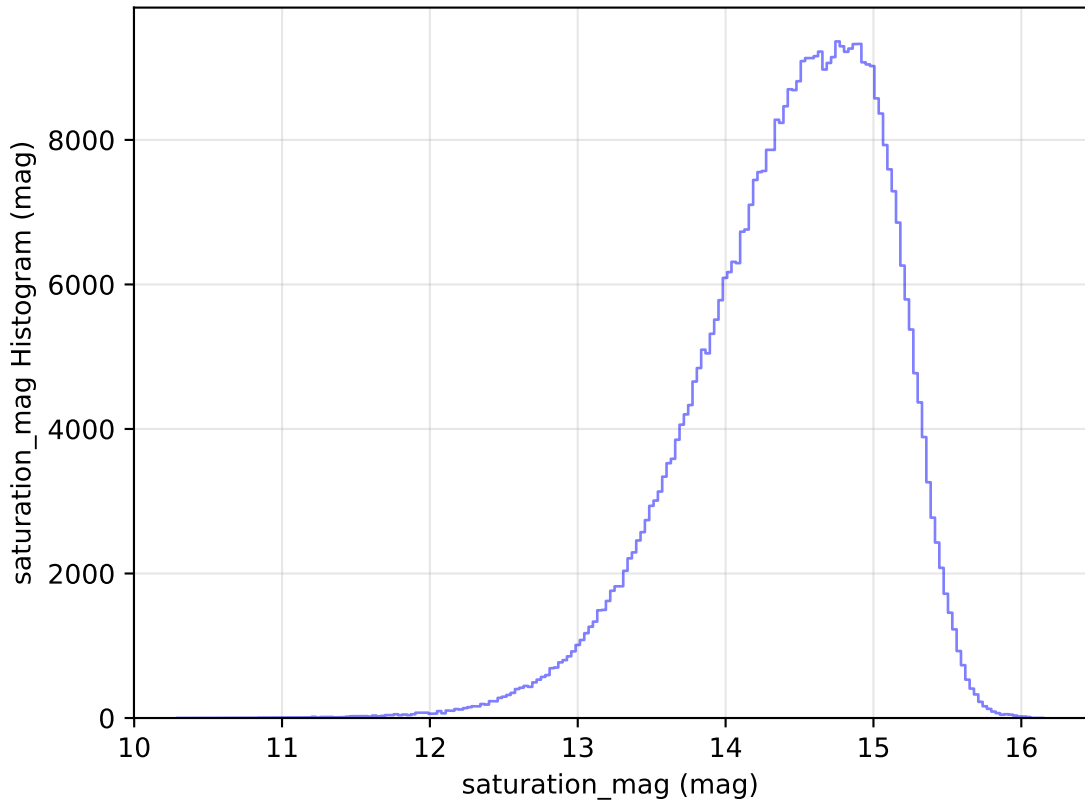
ddf_loaded_half_fl1_v3.4_10yrs All sky i band: saturation_mag Histogram
