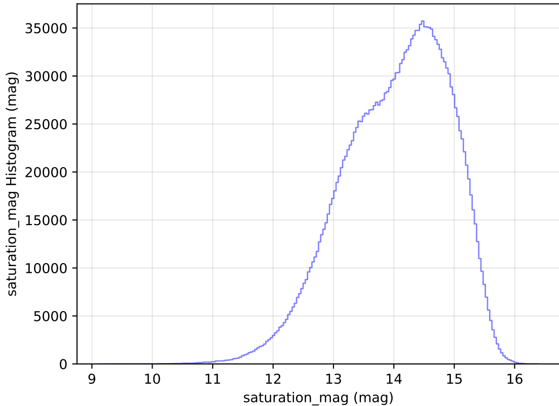
ddf_loaded_half_fl1_v3.4_10yrs All sky all bands: saturation_mag Histogram
