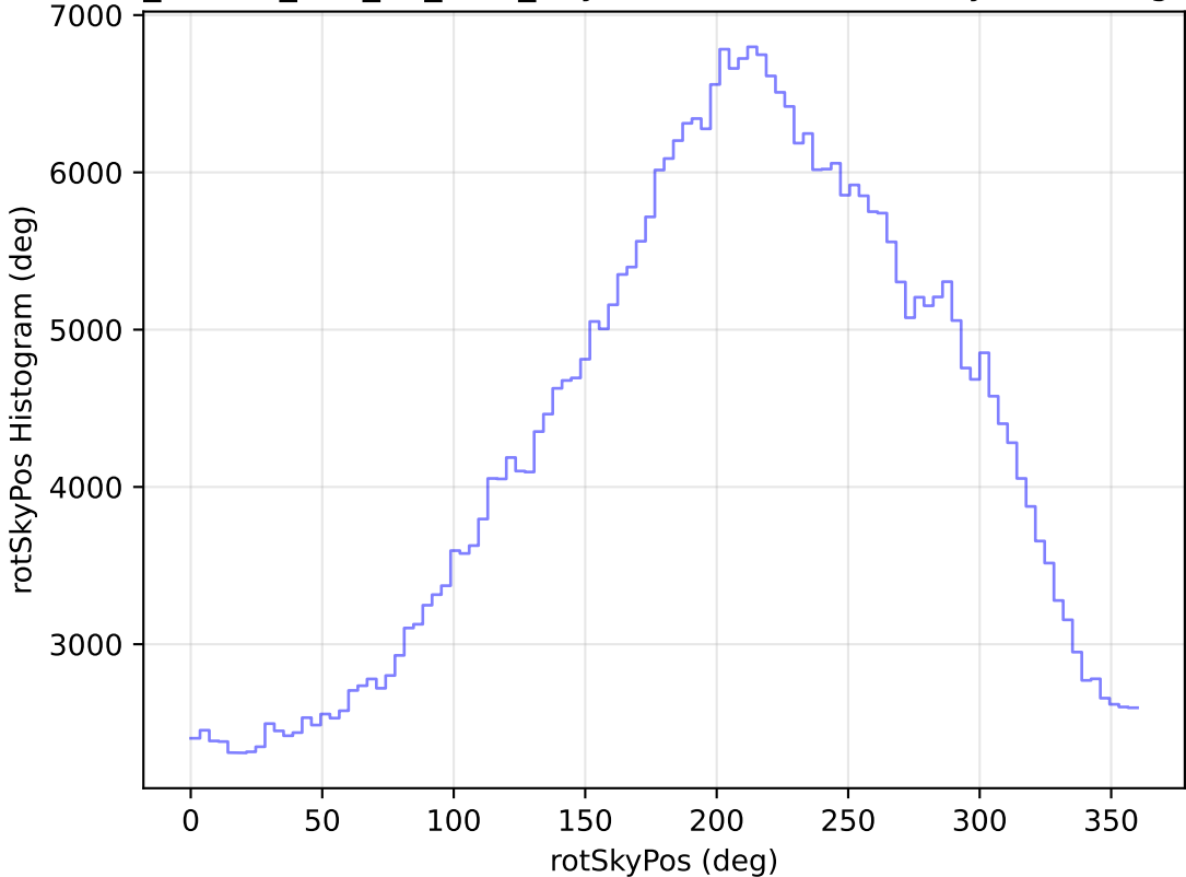
ddf_loaded_half_fl1_v3.4_10yrs WFD z band: rotSkyPos Histogram
