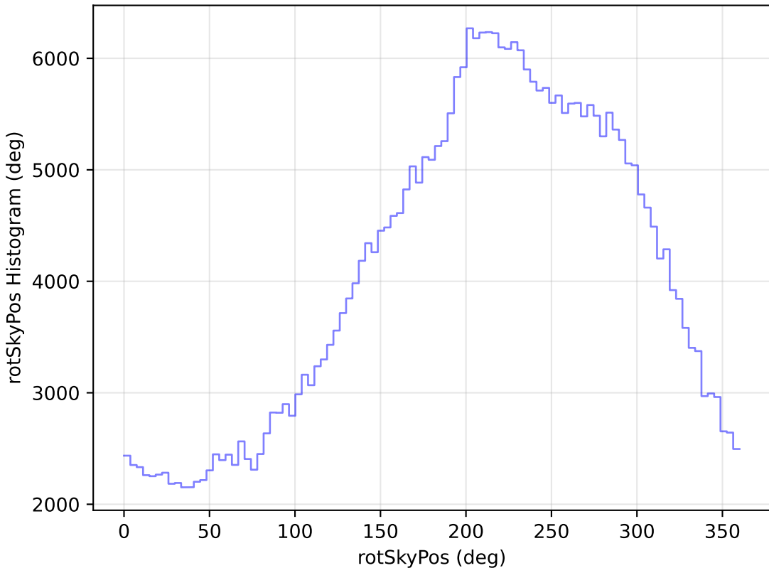
ddf_loaded_half_fl1_v3.4_10yrs WFD y band: rotSkyPos Histogram
