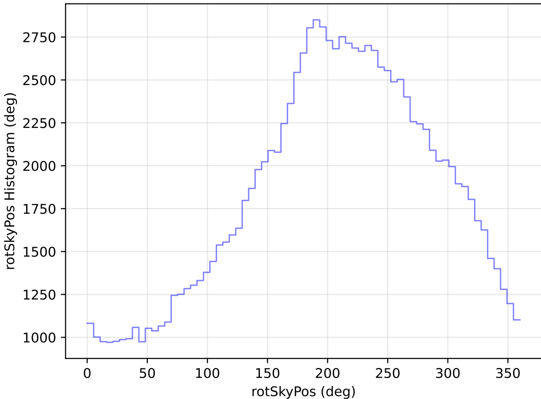
ddf_loaded_half_fl1_v3.4_10yrs WFD u band: rotSkyPos Histogram
