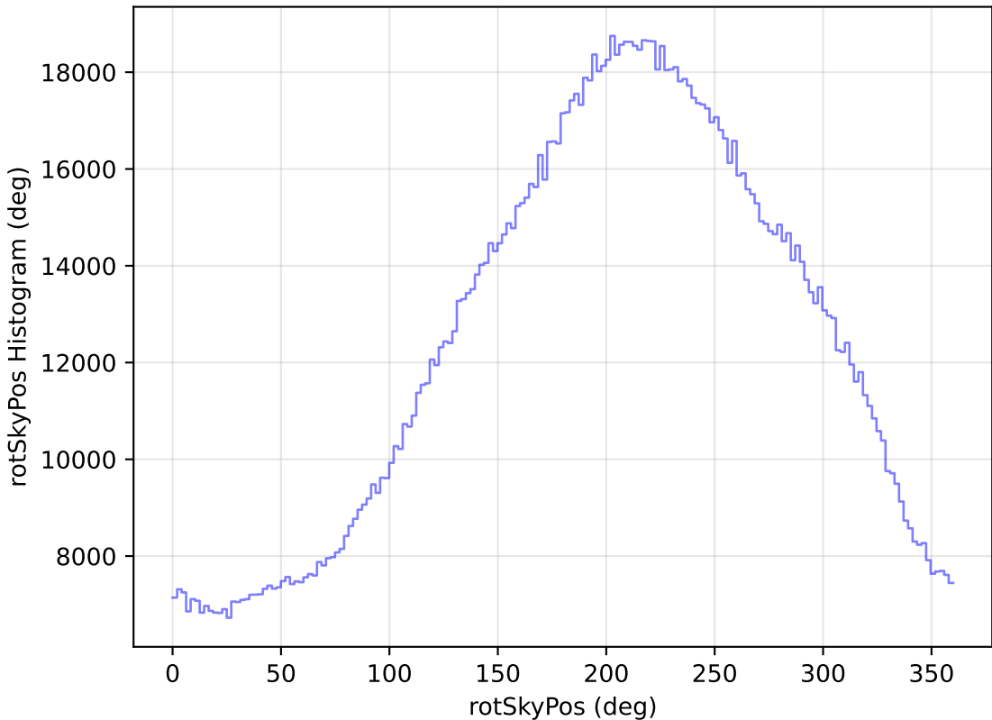
ddf_loaded_half_fl1_v3.4_10yrs WFD all bands: rotSkyPos Histogram
