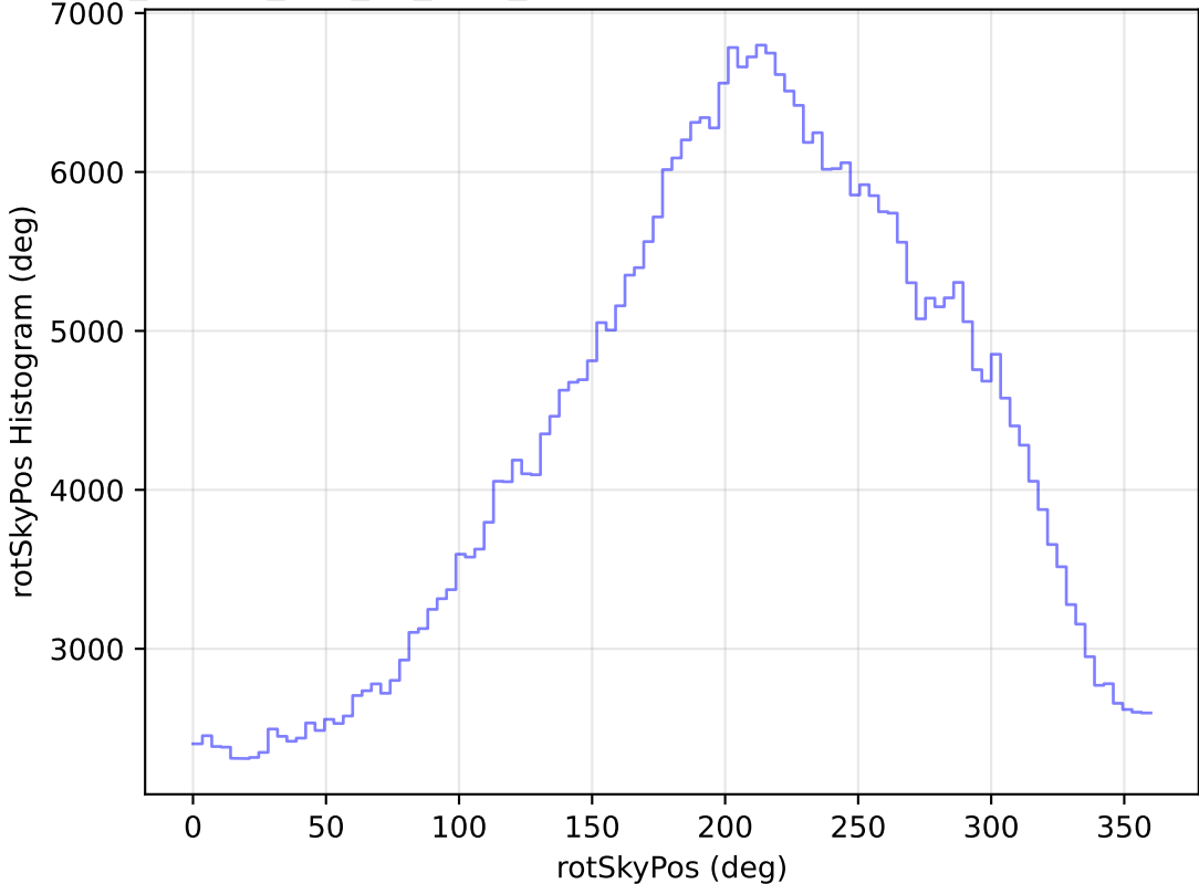
ddf_loaded_half_fl1_v3.4_10yrs All sky z band: rotSkyPos Histogram
