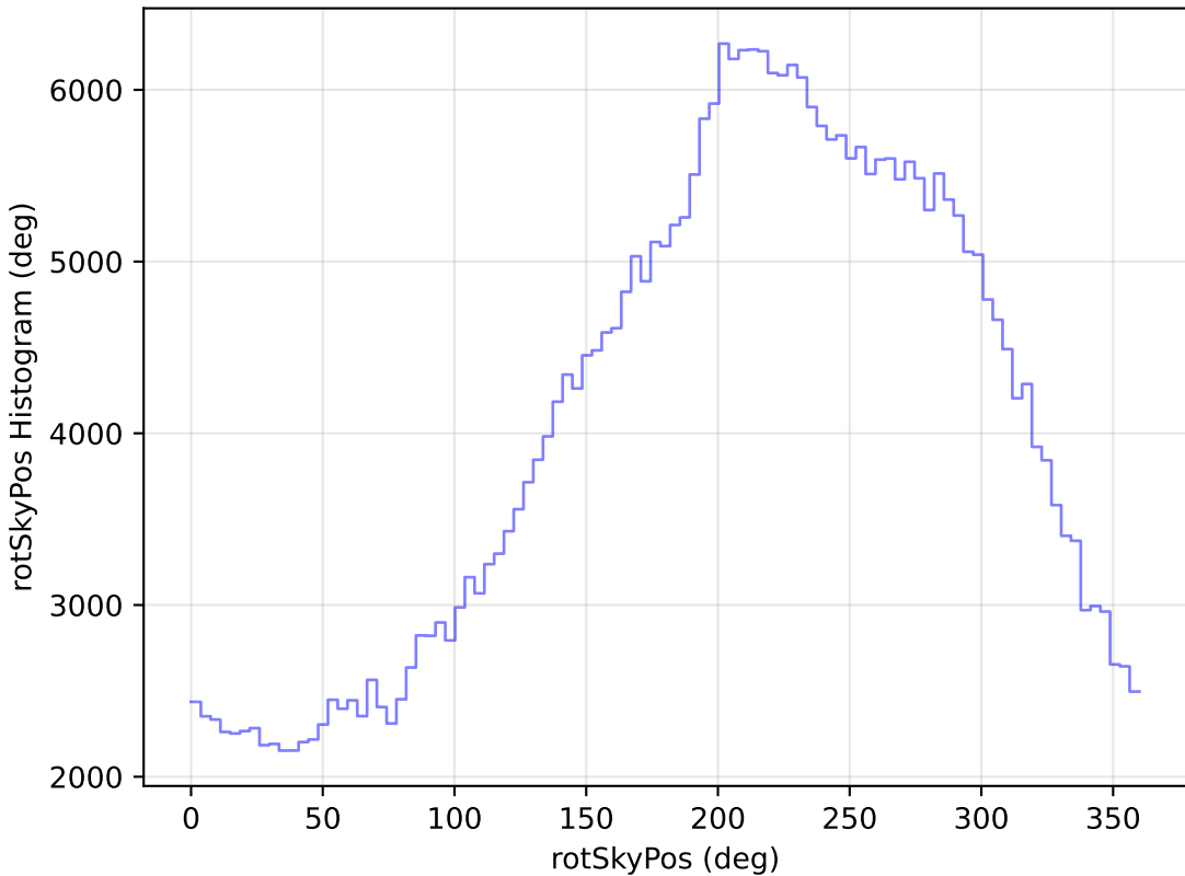
ddf_loaded_half_fl1_v3.4_10yrs All sky y band: rotSkyPos Histogram
