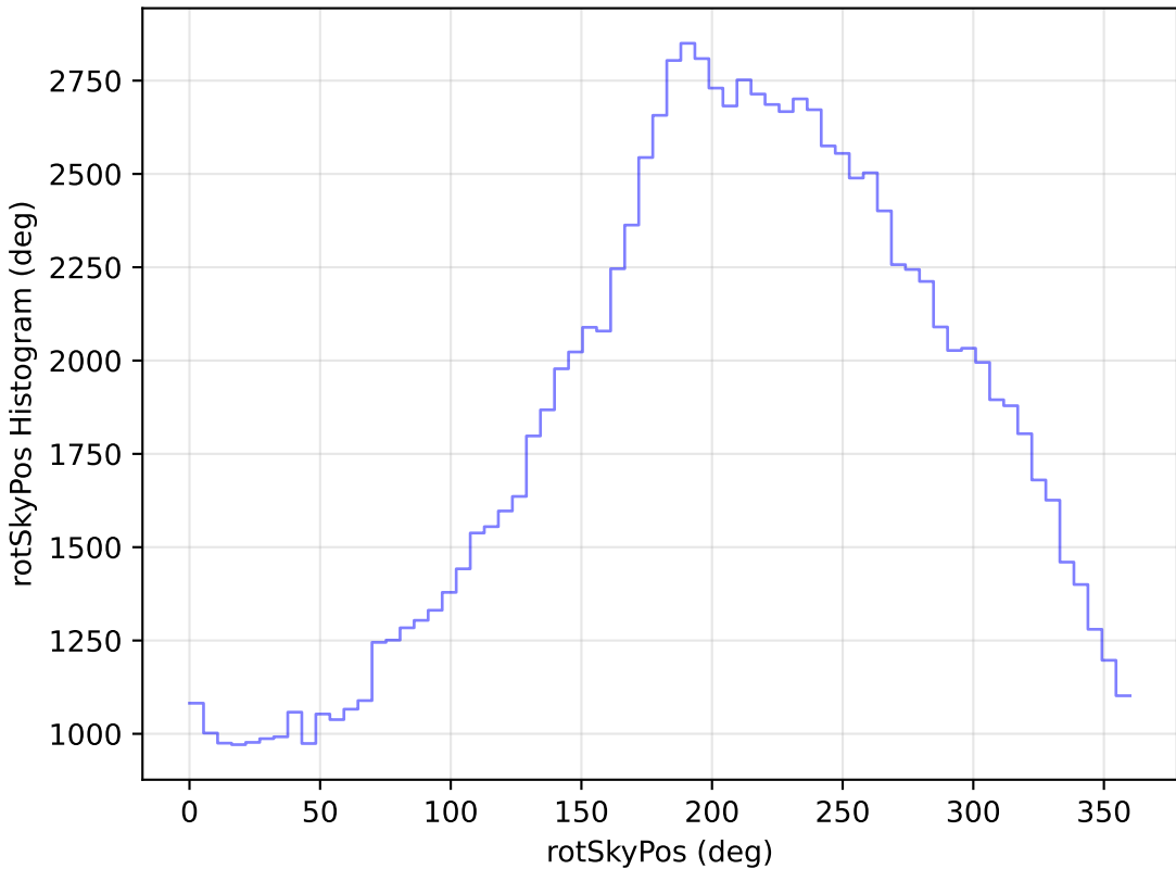
ddf_loaded_half_fl1_v3.4_10yrs All sky u band: rotSkyPos Histogram
