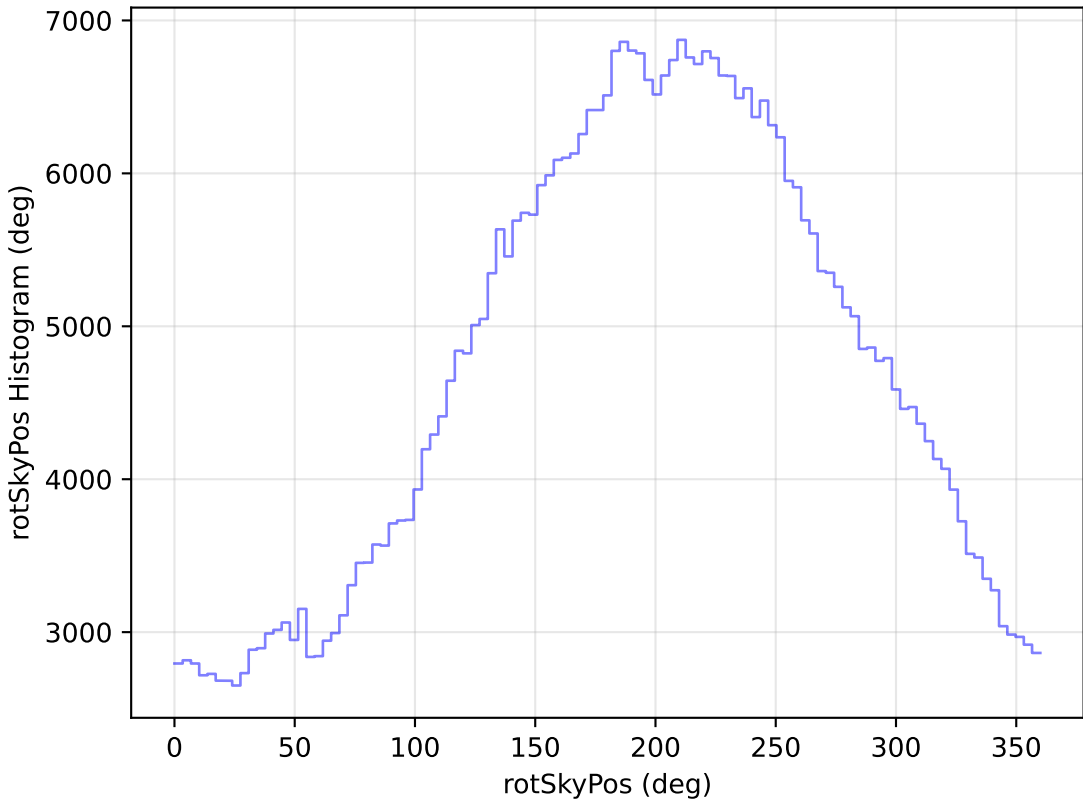
ddf_loaded_half_fl1_v3.4_10yrs All sky r band: rotSkyPos Histogram
