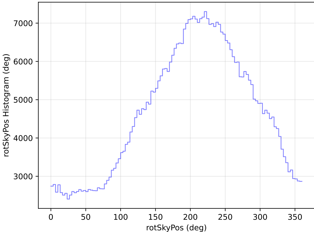
ddf_loaded_half_fl1_v3.4_10yrs All sky i band: rotSkyPos Histogram
