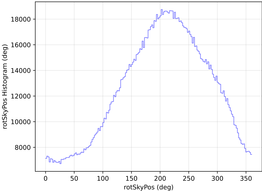
ddf_loaded_half_fl1_v3.4_10yrs All sky all bands: rotSkyPos Histogram
