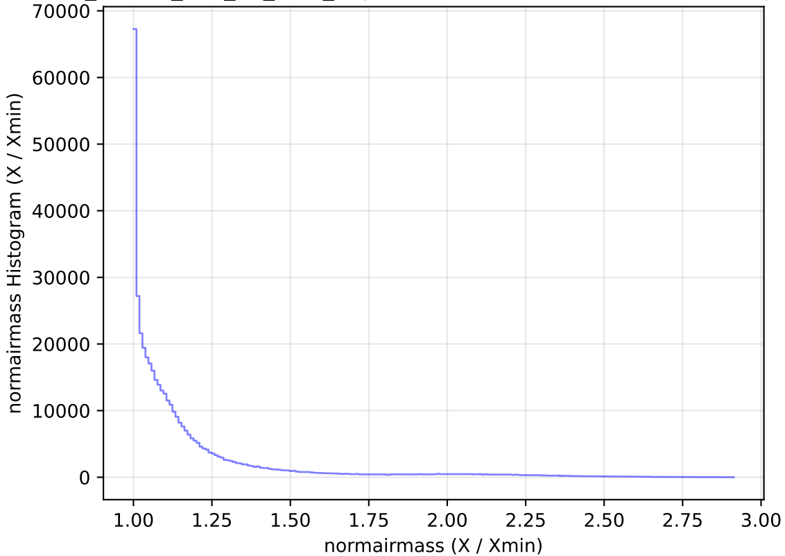
ddf_loaded_half_fl1_v3.4_10yrs WFD z band: normairmass Histogram
