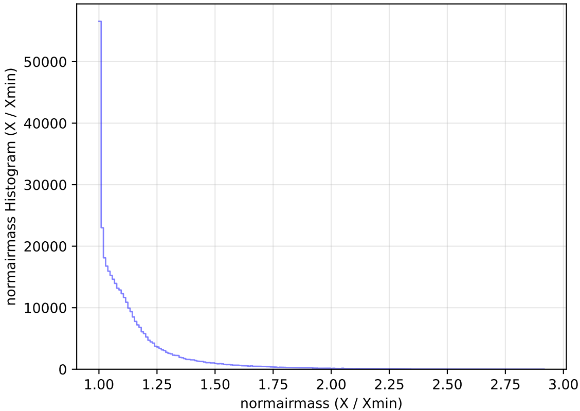
ddf_loaded_half_fl1_v3.4_10yrs WFD y band: normairmass Histogram
