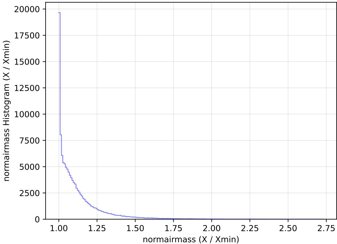
ddf_loaded_half_fl1_v3.4_10yrs WFD u band: normairmass Histogram
