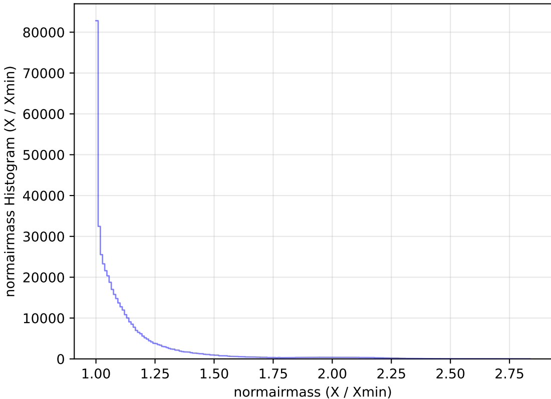
ddf_loaded_half_fl1_v3.4_10yrs WFD r band: normairmass Histogram
