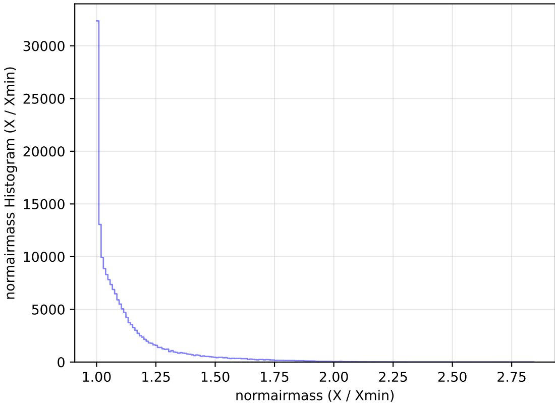
ddf_loaded_half_fl1_v3.4_10yrs WFD g band: normairmass Histogram
