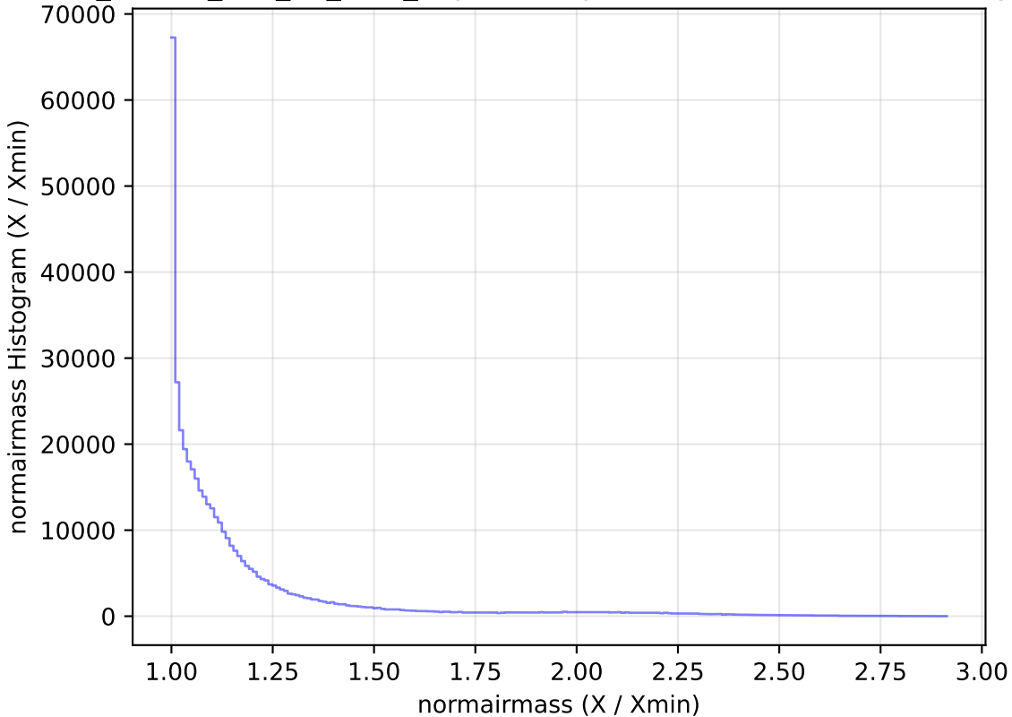
ddf_loaded_half_fl1_v3.4_10yrs All sky z band: normairmass Histogram
