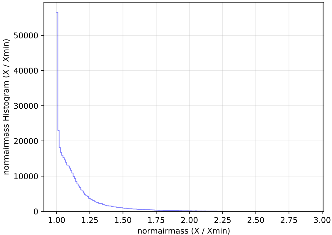
ddf_loaded_half_fl1_v3.4_10yrs All sky y band: normairmass Histogram
