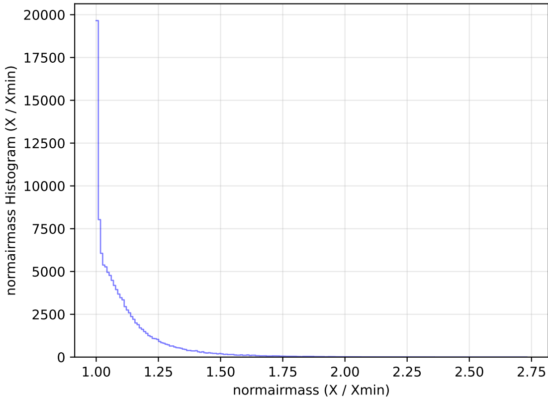
ddf_loaded_half_fl1_v3.4_10yrs All sky u band: normairmass Histogram
