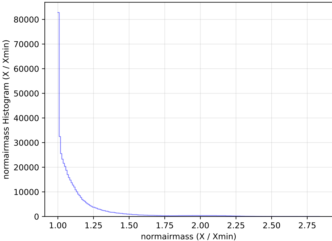
ddf_loaded_half_fl1_v3.4_10yrs All sky r band: normairmass Histogram
