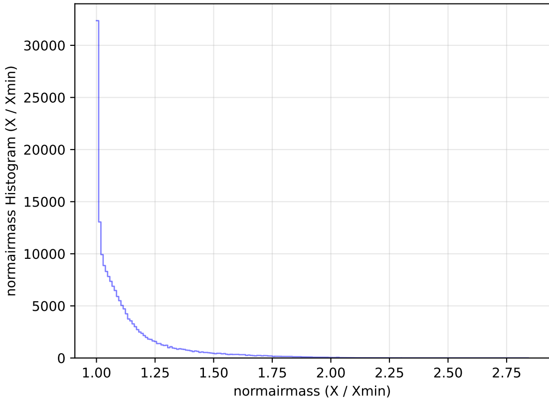
ddf_loaded_half_fl1_v3.4_10yrs All sky g band: normairmass Histogram
