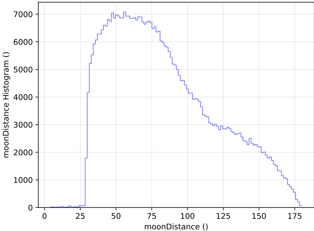
ddf_loaded_half_fl1_v3.4_10yrs WFD z band: moonDistance Histogram
