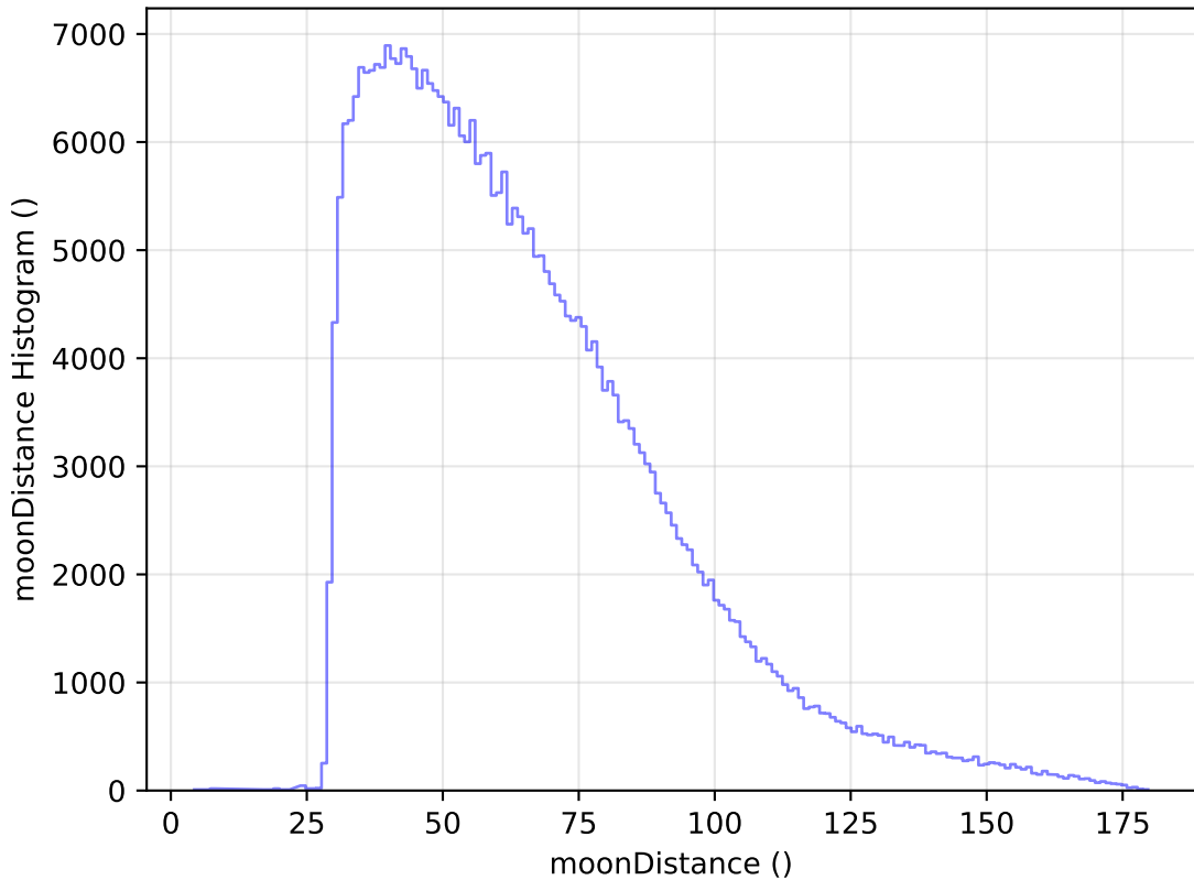
ddf_loaded_half_fl1_v3.4_10yrs WFD y band: moonDistance Histogram
