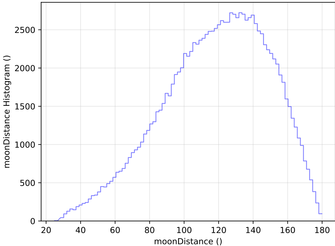
ddf_loaded_half_fl1_v3.4_10yrs WFD u band: moonDistance Histogram
