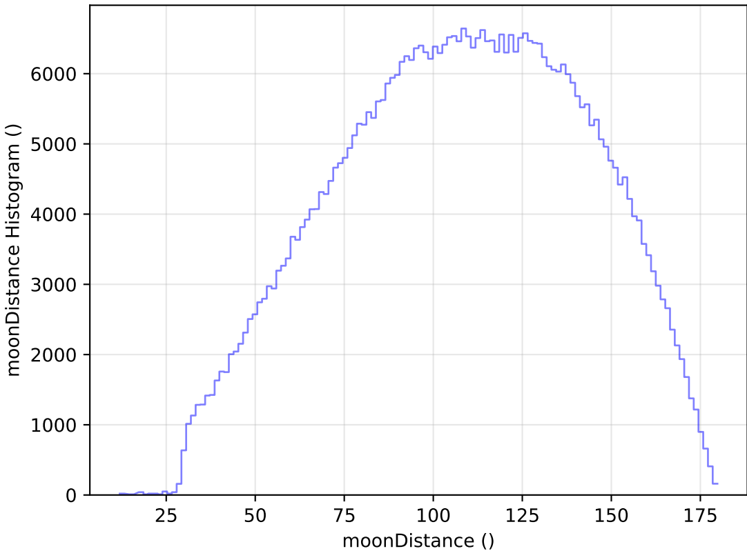
ddf_loaded_half_fl1_v3.4_10yrs WFD r band: moonDistance Histogram
