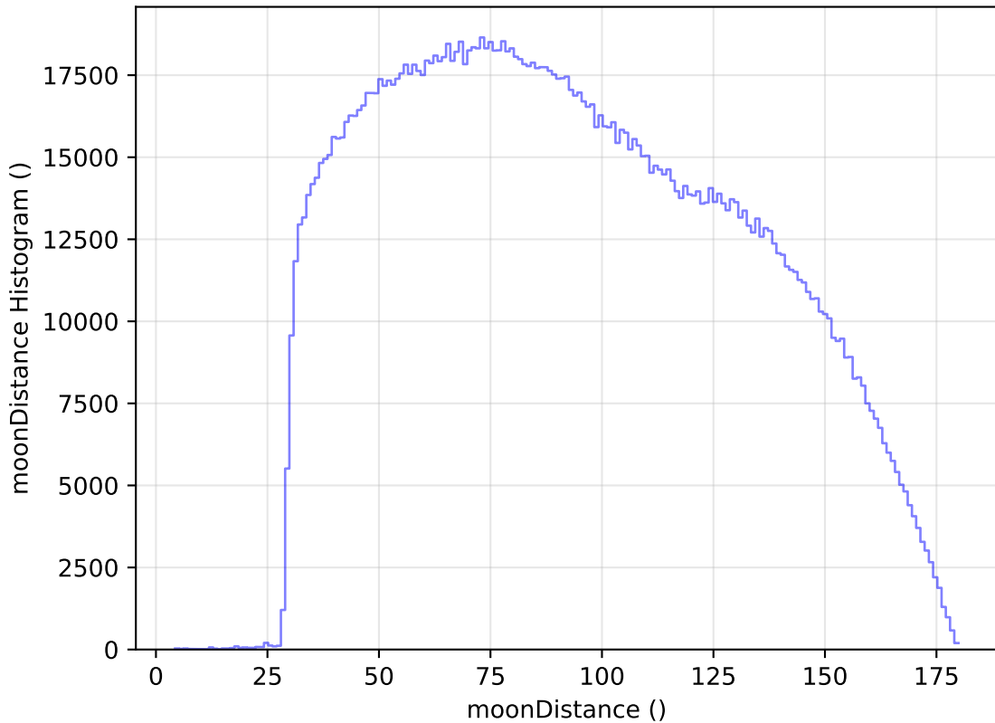
ddf_loaded_half_fl1_v3.4_10yrs WFD all bands: moonDistance Histogram
