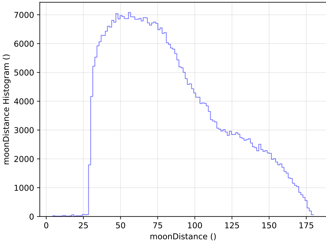
ddf_loaded_half_fl1_v3.4_10yrs All sky z band: moonDistance Histogram
