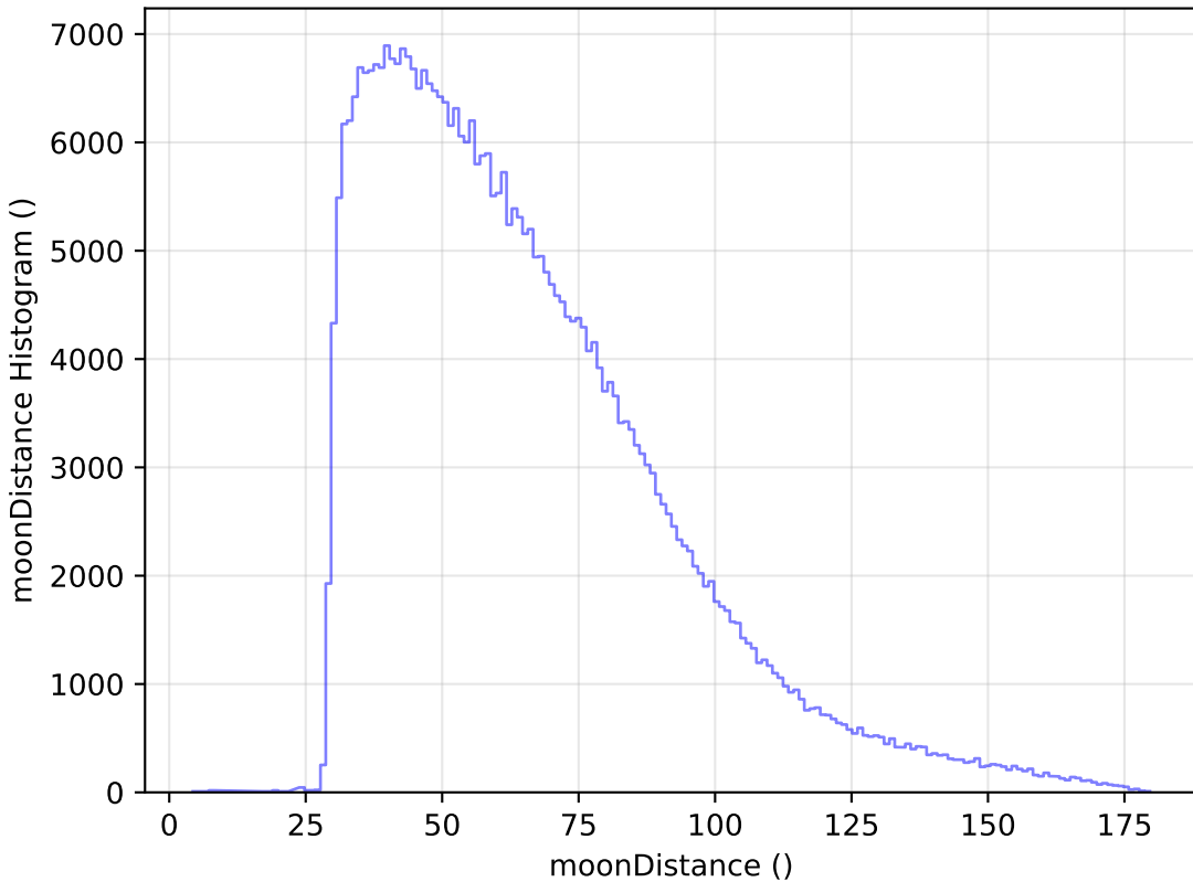
ddf_loaded_half_fl1_v3.4_10yrs All sky y band: moonDistance Histogram
