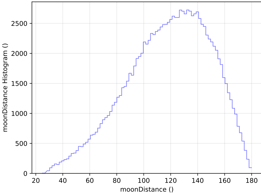
ddf_loaded_half_fl1_v3.4_10yrs All sky u band: moonDistance Histogram
