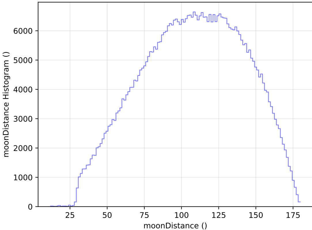
ddf_loaded_half_fl1_v3.4_10yrs All sky r band: moonDistance Histogram
