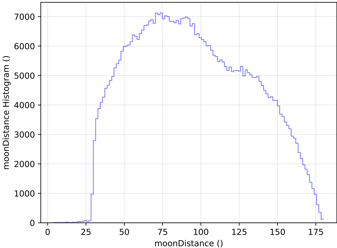
ddf_loaded_half_fl1_v3.4_10yrs All sky i band: moonDistance Histogram
